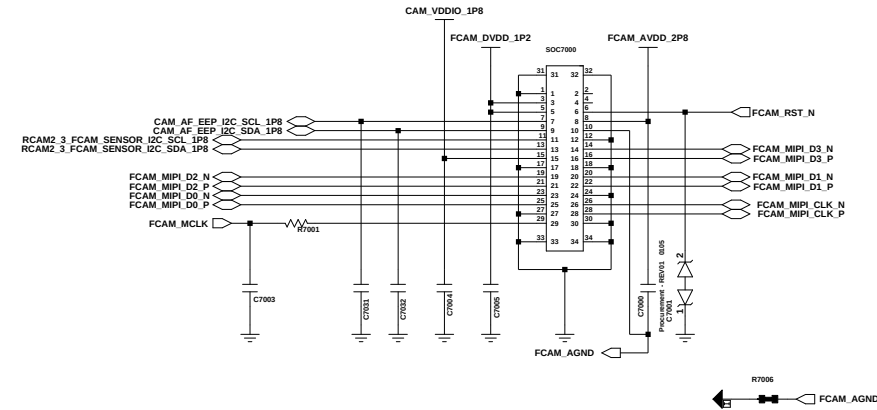
FRONT_8M_FF (30PIN)_GC08A3
