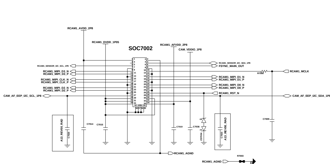
RCAM1_50M(34PIN)_S5KJN1
