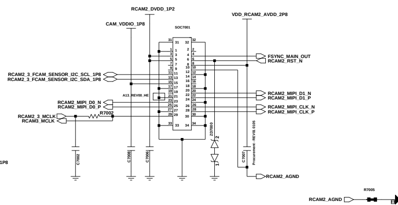
RCAM2_5M_UW (30pin)_GC5035
