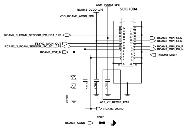
RCAM3_2M_BOKEH (24PIN)_GC02M1B
